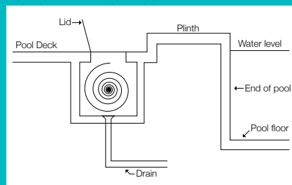
Commercial Hideaway System Behind Plinth. Deck Mount
