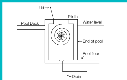
Commercial Hideaway System Under Plinth
