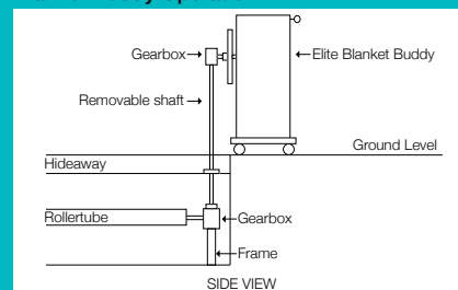
Commercial Hideaway System Blanket Buddy Operation.
